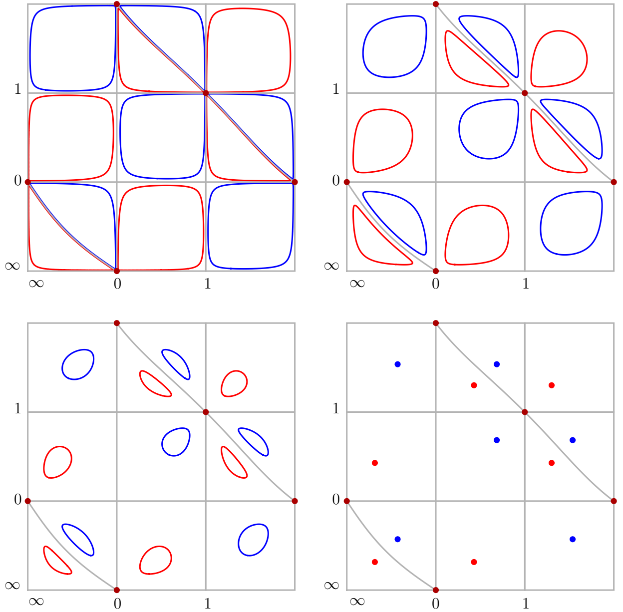
Figure 1: These are plots of the curves F_+ = 0 , in red, and F_- = 0 , in blue, for real (\sigma, \tau) as \psi^5 ranges from 0 to 1. The diagram is misleading with respect to the points (1, 1) , (0, \infty) and (\infty, 0) which lie on the curve for all \psi but for \psi \neq 0 the neighborhoods of the curve on which they lie intersect the plane on which (\sigma, \tau) are both real only in points. The figures show also the images of the 10 exceptional curves of dP_5 . These are the 3 points (1, 1) , (0, \infty) and (\infty, 0) together with the 7 lines \sigma = 0, 1, \infty , \tau = 0, 1, \infty and \sigma\tau = 1 . After resolution, the exceptional curves corresponding to the points (1, 1) , (0, \infty) and (\infty, 0) intersect each of the curves F_{\pm} = 0 in two points. So too do the other exceptional curves, though the intersections are in complex points not visible in the figure. The resolved curves are smooth apart from the cases \psi^5 = 0, 1, \infty . As \psi \rightarrow 0 the curves tend to the exceptional lines of dP_5 and, as \psi \rightarrow 1 , the curves F_{\pm} = 0 each develop 6 nodes corresponding to the limiting points shown in the final figure.
