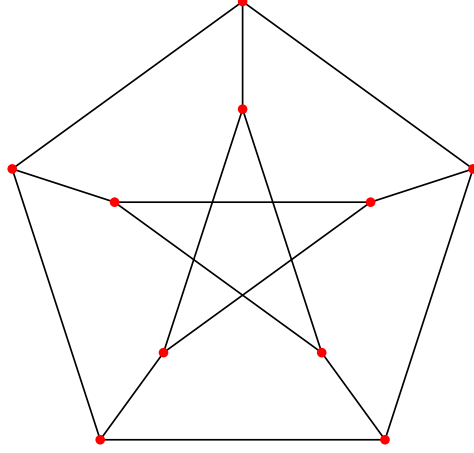
Figure 2: The Petersen graph, which summarizes the combinatorics of the intersections of the exceptional divisors E_{ij} . In the figure, the exceptional divisors correspond to vertices and their intersections correspond to the edges.
